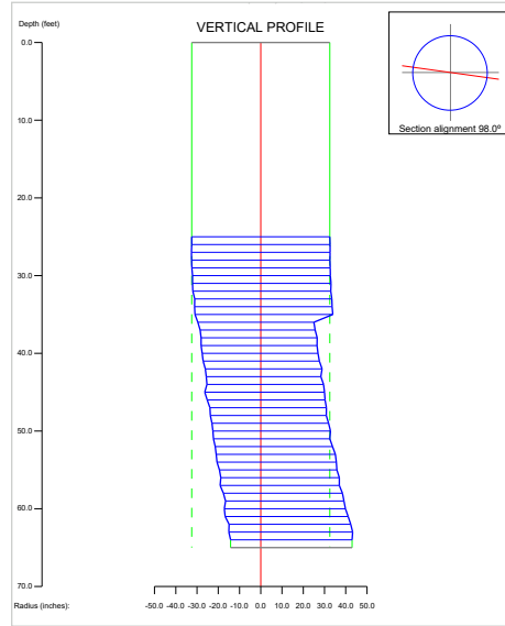
Figure 1 – SONICaliper profile - pass 1
