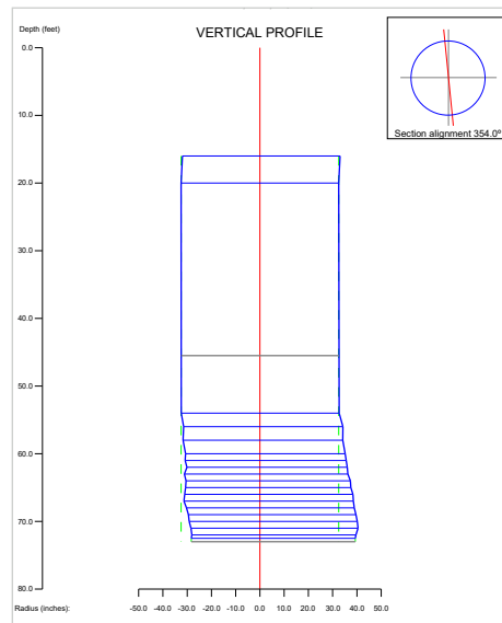
Figure 3 – SONICaliper profile - pass 6
