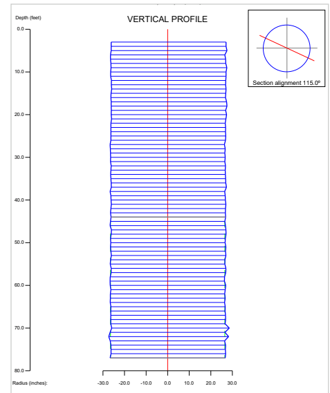
Figure 4 – SONICaliper profile – grout monitoring
