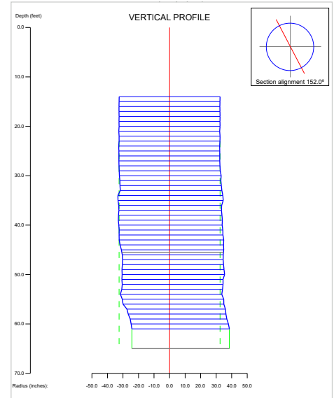
Figure 2 – SONICaliper profile - pass 3
